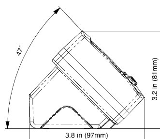
Side view desk mount with battery compartment
